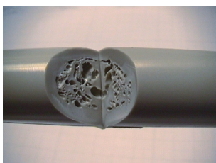
Fig. 3: Motorbike hinged tie bar
